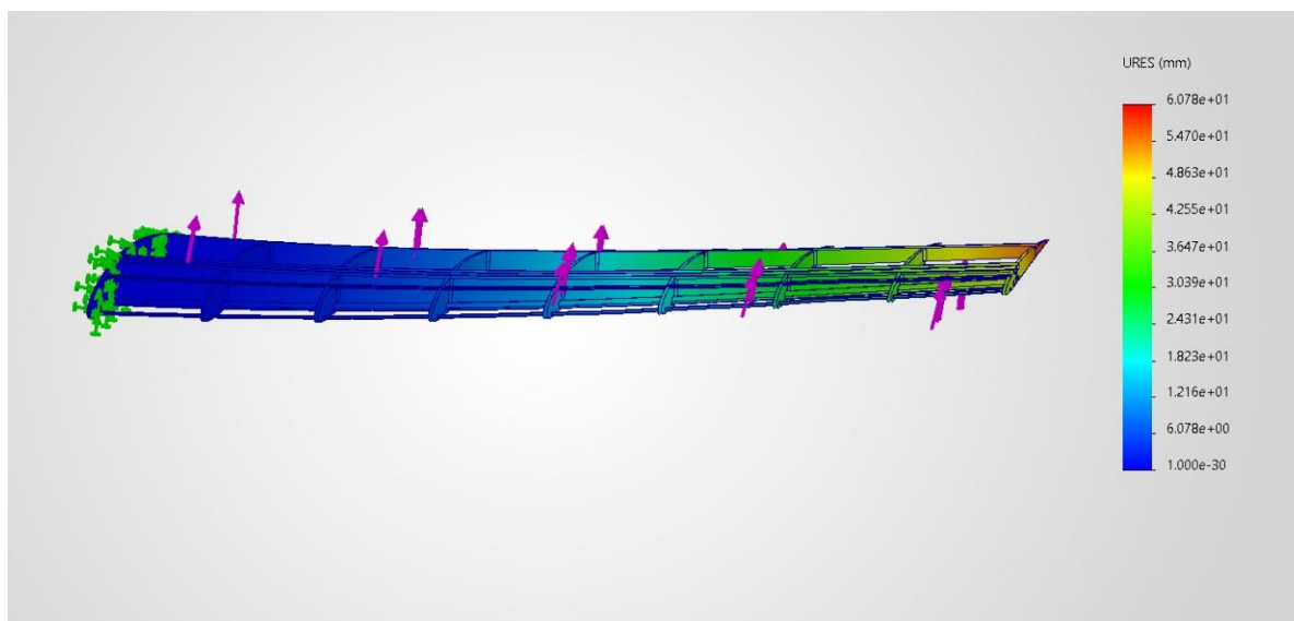
Figure 4. CFRP-like spar displacement under identical loading.
