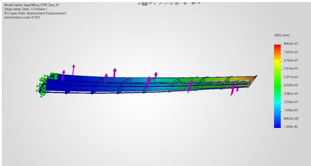
Figure 3. Baseline displacement under 5,000 N test load.
